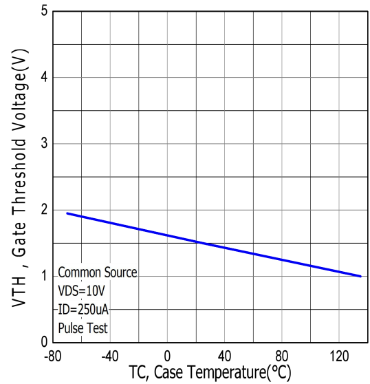
Figure.10 Typical Threshold Voltage vs Case Temperature
