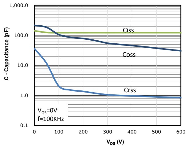
Fig 19: Capacitance Characteristics
