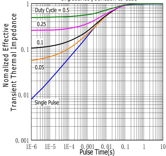
Figure.11 Maximum Effective Thermal Impedance, Junction to Case
